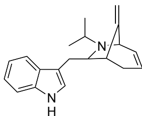
peduncularine
