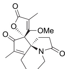
(±)-stemonamide
