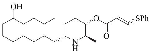
Uoamines A (E) and B (Z)
