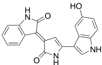
violacein
