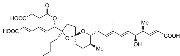
(-)-reveromycin B
