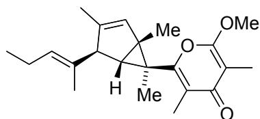
(±)-photodeoxytridachione
