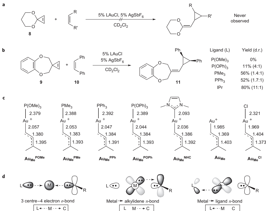
Figure 3 | Experimental and theoretical comparison for the carbene reactivity of the substrate with different ancillary ligands. a,b , Attempted ( a ) and observed ( b ) carbene-like reactivity, demonstrating the impact of the ancillary ligand on the yield of cyclopropanation product. c , Bond distances in \text{Au}_{\text{Me}}^{\text{L}} complexes. d , A stylized depiction of the most important bonding interactions in \text{L-Au(i)-CR}_2^+ species. d.r., diastereomeric ratio.
