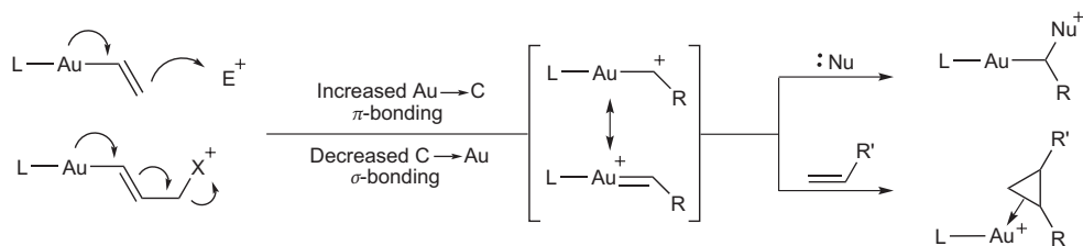
Figure 4 | Arrow pushing in the formation of gold-stabilized carbenes. Such arrow pushing is a useful mnemonic for keeping track of electrons, but it can lead to misconceptions about bonding. Although the gold-carbon bond in the intermediate carbene has both \sigma and \pi components, the overall bond order is generally less than or equal to one.
