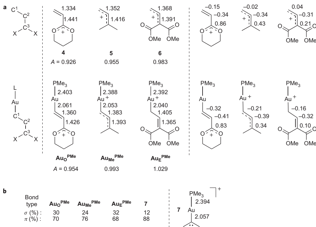
Figure 2 | Structural and electronic comparison of cationic metal-free and [\text{AuPMe}_3]^+ substituted substrates. a , On the left, calculated bond distances (Å), and on the right, natural charges for C 1 , C 2 , and C 3 . Parameter A is defined as the ratio of bond distances (C 1 -C 2 )/(C 2 -C 3 ) and correlates to the polarization of the \pi -electrons along the delocalized C 1 -C 2 -C 3 system. b , A comparison with gold alkylidene 7 showing the relative natural orbital populations of \sigma and \pi contributions to the gold-carbon bond. Calculated bond distances (Å) for 7 are shown on the right.
