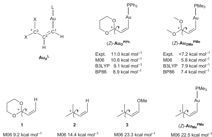
Figure 1 | Calculated and experimental activation energies to bond rotation (indicated with arrows). C 3 -C 2 bond rotation barriers are decreased when C 3 is substituted with carbocation-stabilizing oxygen atoms. Throughout this article, gold complexes will be referred to according to the \text{Au}_X^L notation, where L indicates the ancillary ligand on gold and X indicates the C 3 substituents (Me = methyl, O = 1,3-dioxanyl, OMe = methoxy, E = methyl ester). M06, B3LYP and BP86 refer to the specific functional used in density functional theory calculations.
