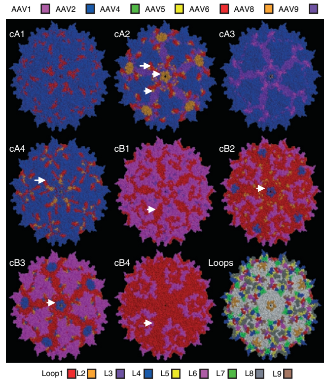
Figure 2 Structural comparison of selected viral chimeras. Molecular models of the adeno-associated virus (AAV) capsid, based on the AAV2 structure, 38 are shown for each chimera along with a model depicting the location of each loop region. Each region is shaded according to the parent serotype from which it was derived, highlighting the substantial sequence variability on exterior regions of the capsid. White arrows indicate important structural regions discussed in text.
