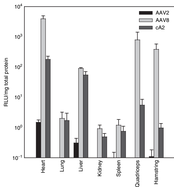
Figure 5 In vivo biodistribution transduction efficiencies of chimera and viral parents. rAAV-Luc vectors ( 10^{11} vector genomes) were delivered via tail vein injections to BALB/c mice ( n = 3 ). For each vector and each tissue analyzed, levels of luciferase expression were normalized to total protein (RLU/mg). AAV, adeno-associated virus; RLU, relative luciferase unit.
