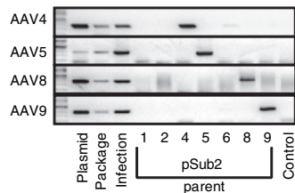
Figure 3 PCR screen of plasmid and viral library. PCRs were performed with serotype-specific primers annealing ~1,400 base pairs (bp) and ~1,700 bp downstream from the cap start codon for the forward and reverse primers, respectively. Positive PCRs yield a band of 200–300 bp in size, depending on the serotype. The plasmid library and vector genome DNA from the packaged virus and passaged virus were analyzed along with the individual parent pSub2 plasmids (labeled 1, 2, 4, 5, 6, 8, and 9). AAV, adeno-associated virus.
