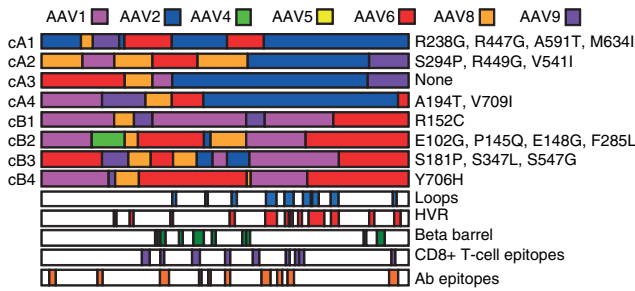
Figure 1 Amino acid sequences of shuffled clones. Graphical representations of the primary protein sequences of each chimera are shown, with the protein segments colored to reflect the parent serotypes from which they were derived. Point mutations present within each sequence are shown next to each clone. Graphical representation of several key viral regions, including surface loops, 38,46,47 hypervariable regions (HVRs), 8 \beta -barrel core, 38 CD8+ T-cell epitopes, 50 and antibody (Ab) epitopes, 15,16 are also depicted to highlight the diversity within these regions. AAV, adeno-associated virus.
