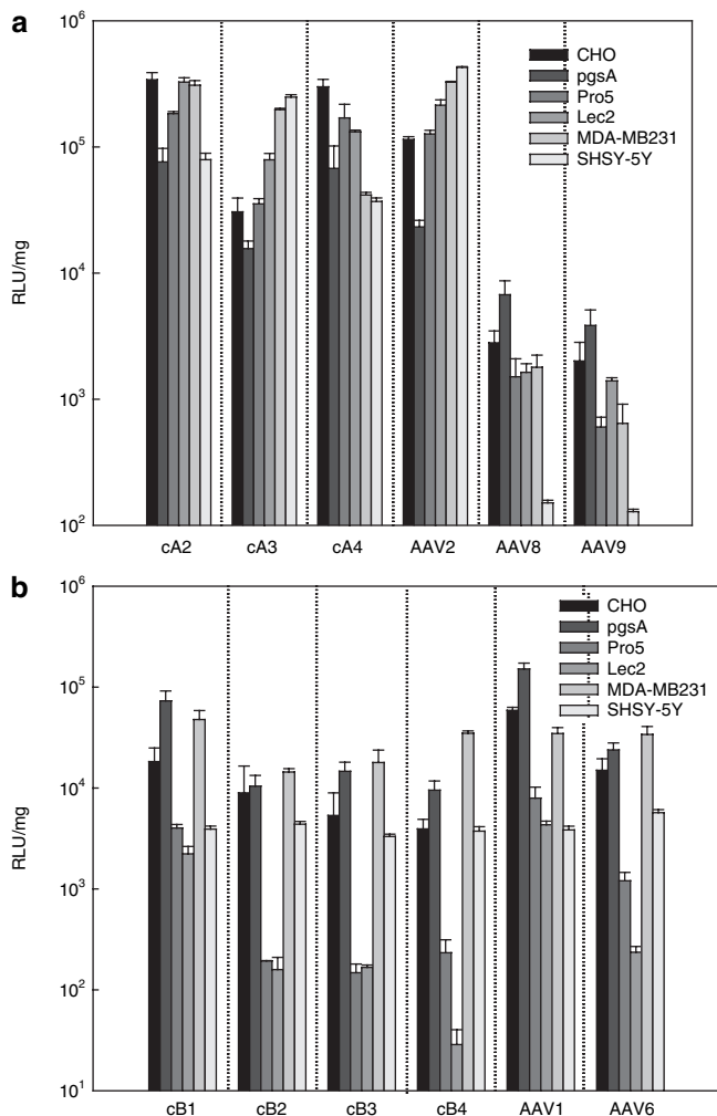
Figure 4 Transduction efficiencies of chimeras and viral parents. rAAV-Luc vectors were used to transduce a panel of cell lines: CHO, pgsA (lacking all GAGs), Pro5, Lec2 (lacking sialic acid), a breast cancer cell line (MDA-MB231), and a neuroblastoma cell line (SHSY-5Y). (a) Relative luciferase signals were normalized to total protein (RLU/mg) for AAV2-related chimeras along with AAV2, 8, and 9 controls ( n = 3 ). (Note: cA1 packaged but was noninfectious.) (b) Normalized relative luciferase values for AAV1/6-related chimeras along with AAV1 and 6 controls are shown ( n = 3 ). AAV, adeno-associated virus; RLU, relative luciferase unit.
