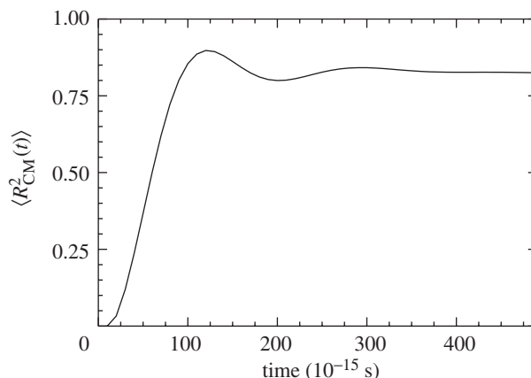
Figure 6. \langle R_{\text{CM}}^2(t) \rangle for VRT(MCY-5r/pol) (solid line) at 298 K. The slope of the curve at t \gg 0 yields the value of the diffusion constant, D .
