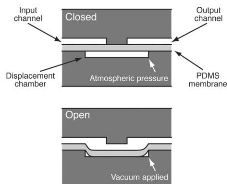
Fig. 1 Monolithic membrane valve structure before, A, and after, B, bonding the wafers together with the PDMS membrane. Valves consist of a discontinuity in a channel (valve seat) directly across the PDMS membrane from an etched displacement chamber. C, Lengthwise cross-section through a valve. Valves are normally closed against low pressures in the valved channels; applying a vacuum to the displacement chamber via the “control” channel pulls the membrane into the displacement chamber and opens the valve.
