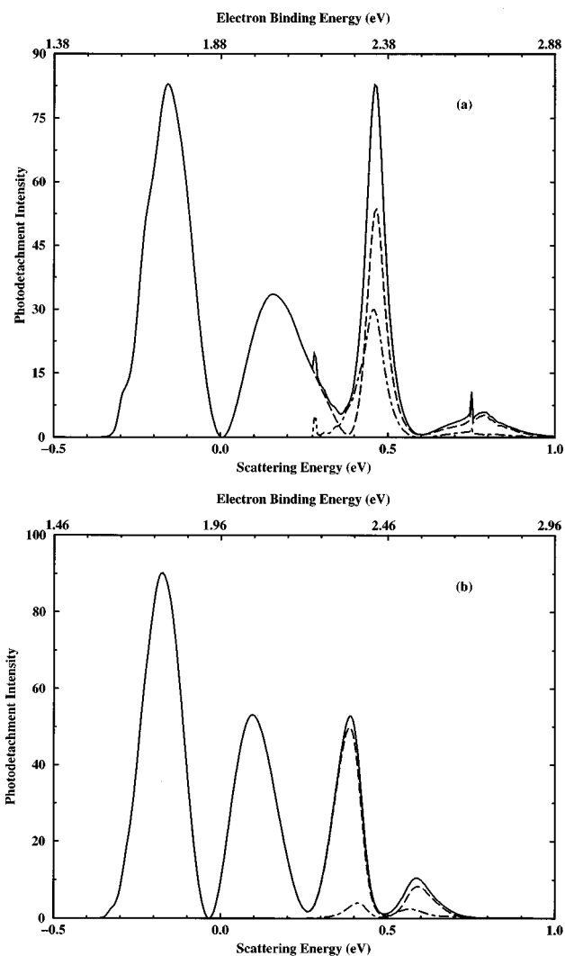
FIG. 3. Same as Fig. 2 but for the \nu=1 state of the anion.
