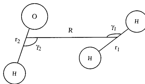
FIG. 1. The reactant Jacobi coordinate system used for the calculations. The dihedral angle, \varphi , (not shown) is the out of plane angle between the \text{OH} and \text{H}_2 bonds.
