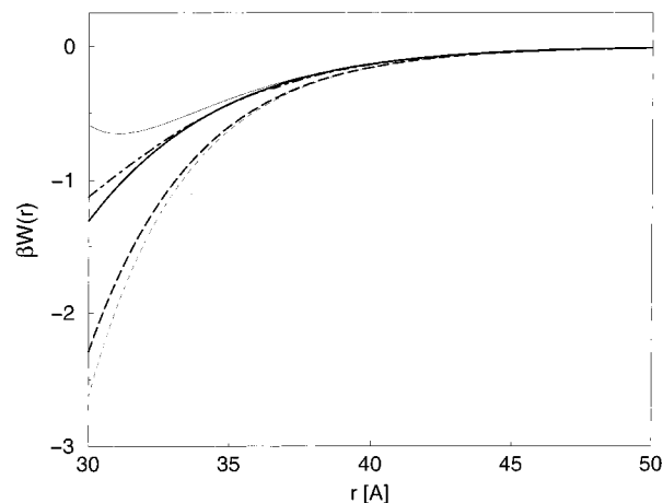
Figure 6. Distance dependence of the intercolloidal potentials of mean force for particles carrying charges q = 8 e_0 and dipoles \mu = 400 D in 0.1 \text{ mol dm}^{-3} univalent electrolyte solution. The macroion diameter \sigma = 3 nm: exact numerical results, eq 8 (thick solid), truncated cumulant expansion, eq 19 (thin solid), perturbation approximation, eq 21 (thick dashed–dotted), additivity approximation based on exact numerical results for distinct charge–dipole and dipole–dipole terms (thick dashed), and additivity approximation based on cumulant expansion approach, eq 13 (thin dashed curve).
