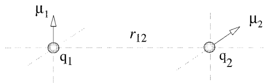
Figure 3. Discrete-orientation model of interacting dipoles (showing orientation \theta_1 = \theta_2 = \theta_{12} = \pi/2 ).
