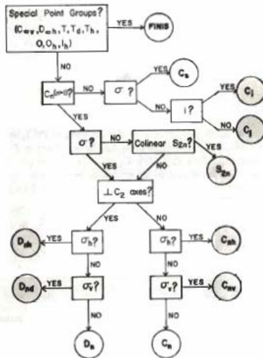
Fig. 1-33. Point group flow chart.
